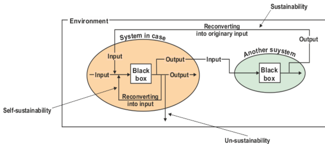
Figure 1. The three cases of an ordered system functioning.
