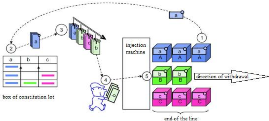
Figure 3.6 Manufacturing mode with Kanban cards fixed batch
