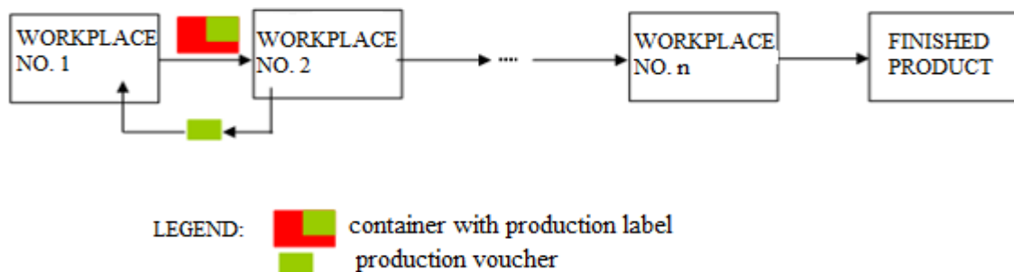
Figure 3.3 Circulation of labels (kanban) and containers
